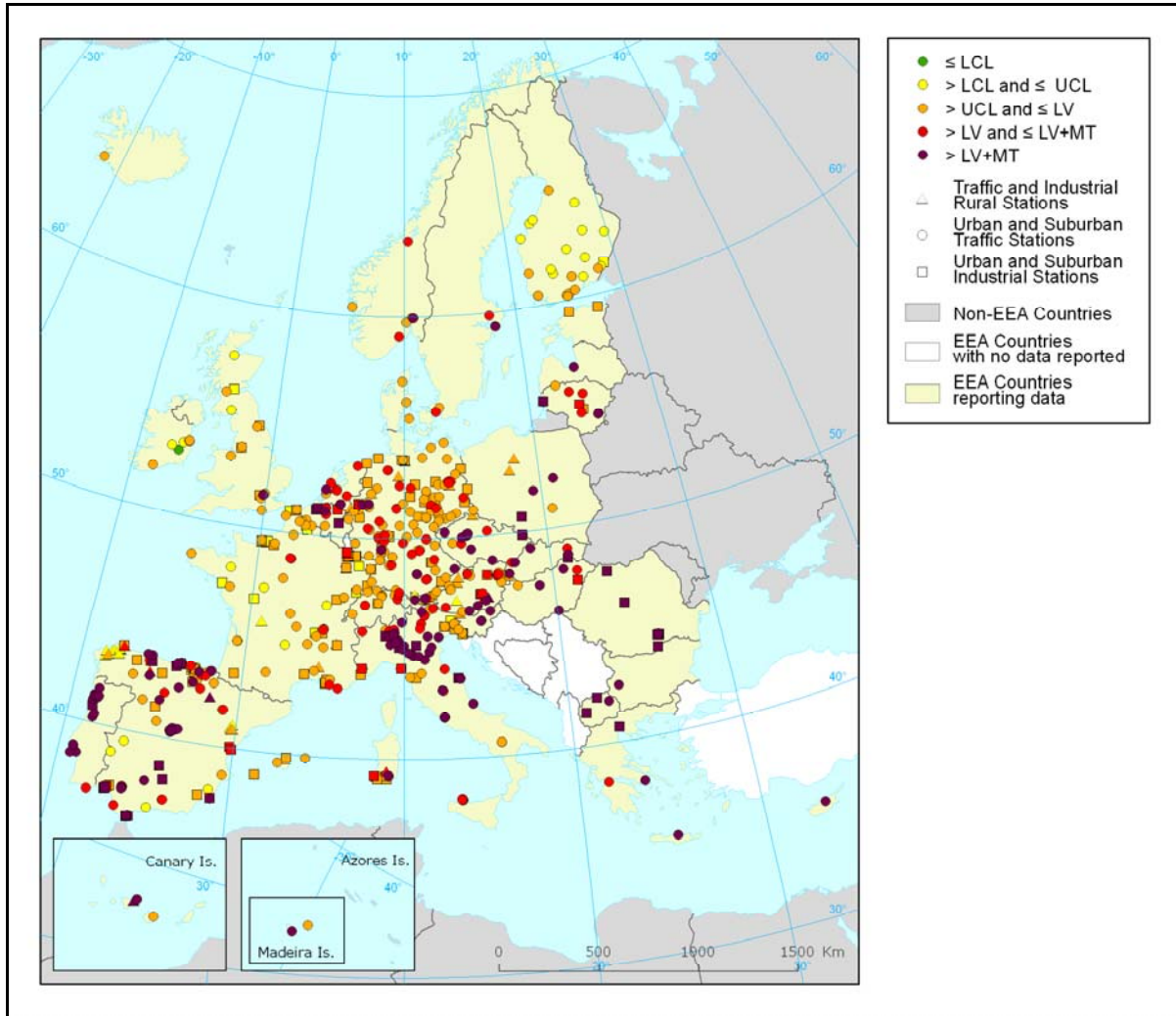
Map with PM10 concentrations at hot spot stations in Europe, 2004, AirBase data
